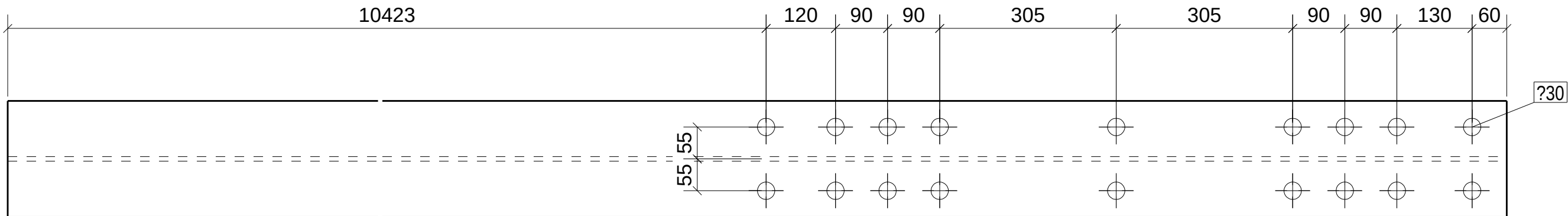
TOP VIEW
